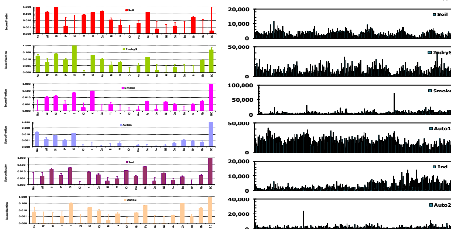
Figure 1. PM 2.5 source apportionment profile at ADMU sampling site. Vehicular emissions making up to 49% of the fine air particulate fraction.
