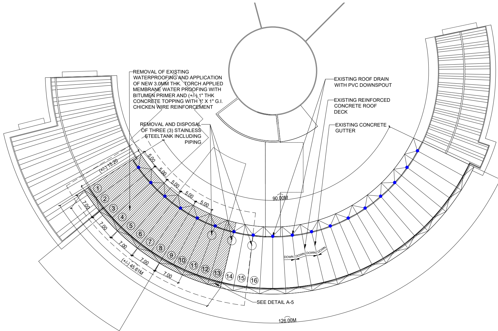
1 ARC BUILDING ROOF FRAMING PLAN A - 5 SCALE NTS
