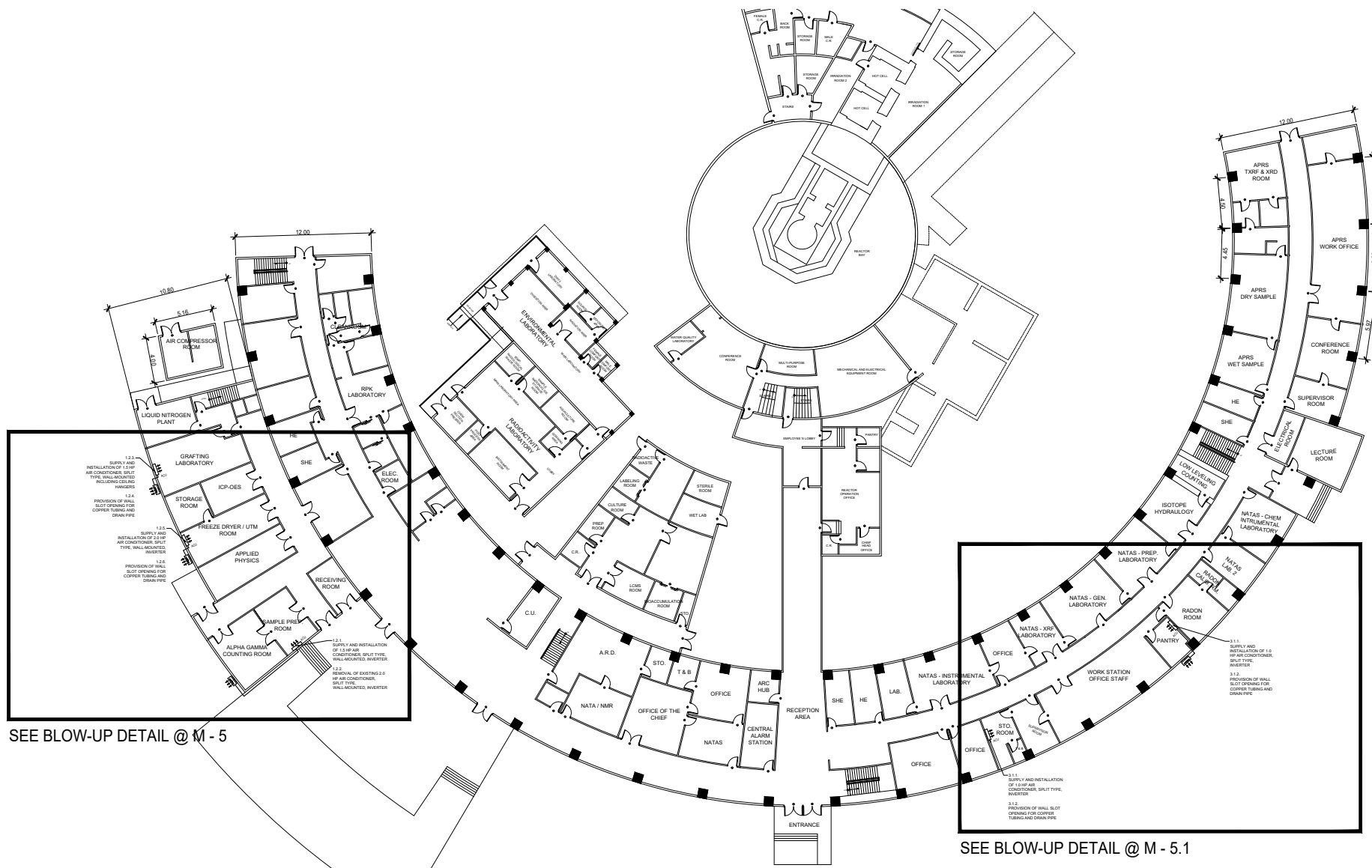
1 GROUND FLOOR LOCATION OF AIR CONDITION UNITS SCALE 1:500 M - 2
