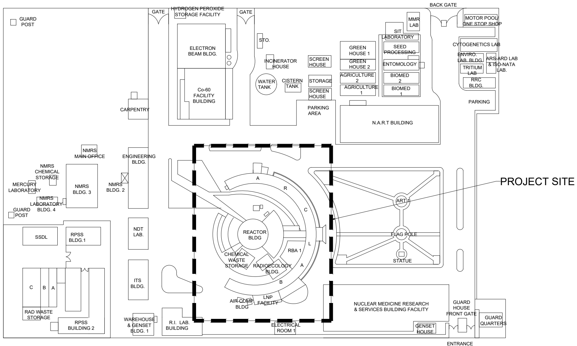
1 ARC BUILDING A - 1 SITE DEVELOPMENT PLAN SCALE NTS
