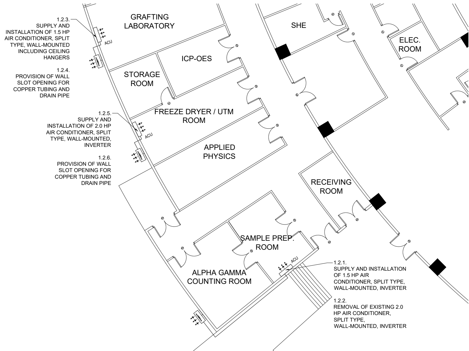
1 GROUND FLOOR, (BLOW-UP 1) M - 5 LOCATION OF AIR CONDITION UNITS SCALE 1:150
